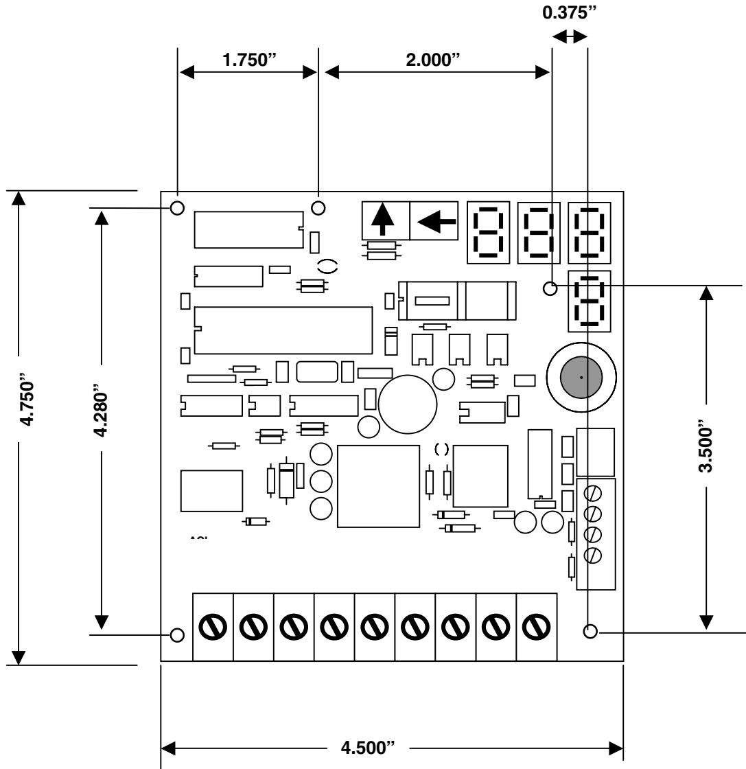
Figure 22 – ECS-100 Controller Board Dimensions
