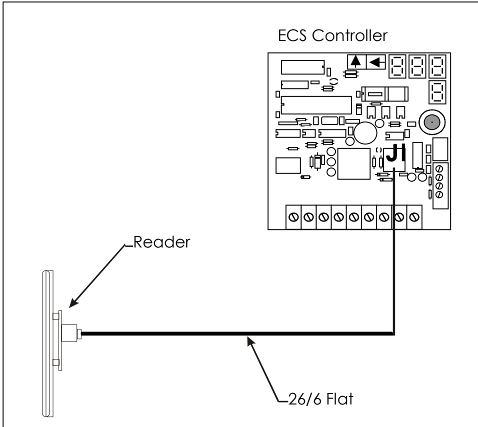
Figure 13 - ComKey Reader to Controller Connection
