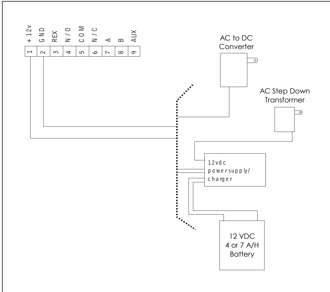
Figure 19 - Available power sources and wiring
