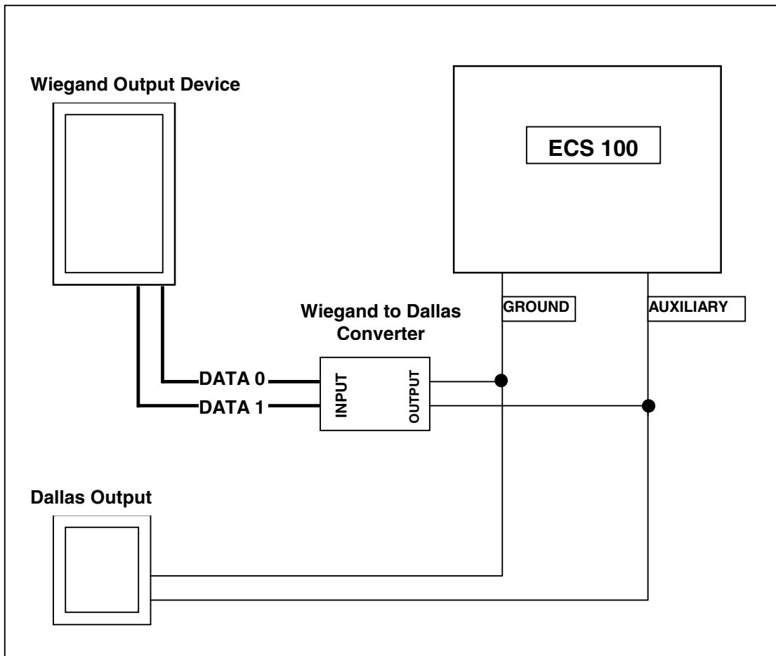
Figure 14 - Wiegand Output Reader to Controller Connection
