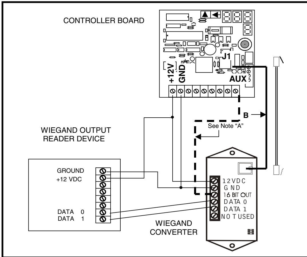
Figure 15 - ECS Wiegand-to-Dallas Converter Connections
