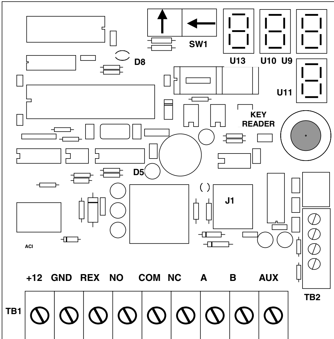
Figure 21 – ECS Controller Board with Component Logic
