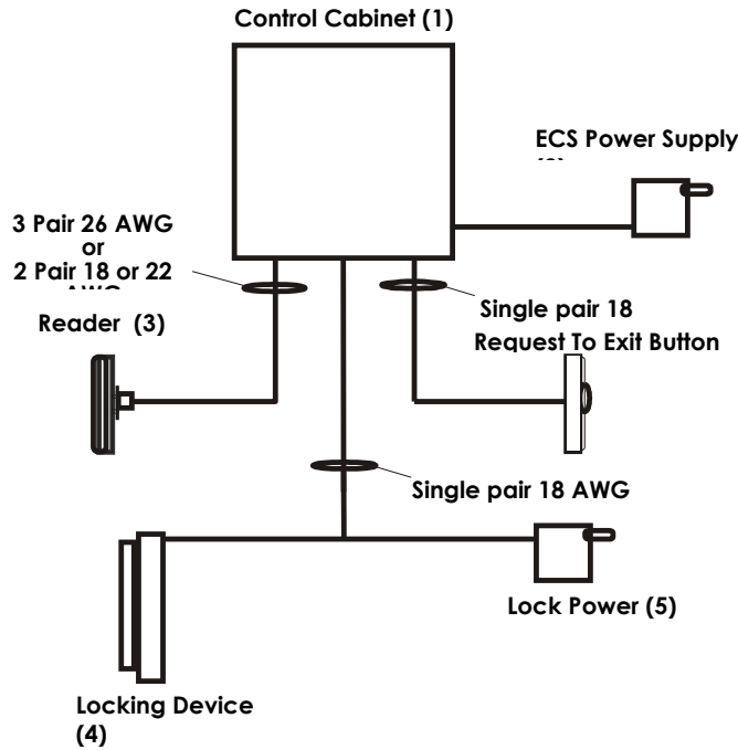
Figure 5 - Installation Block Diagram
