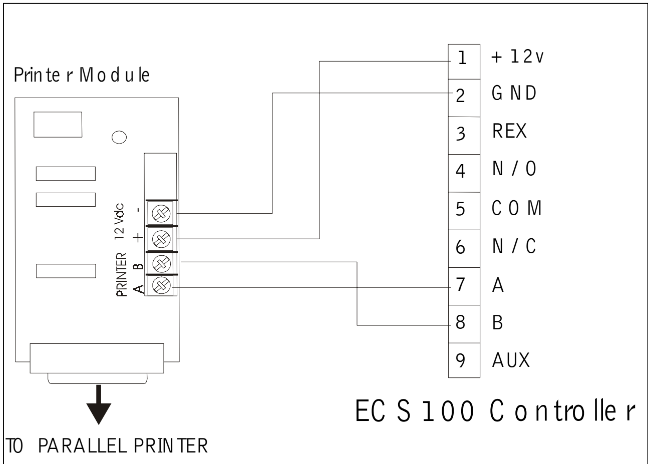
Figure 17 - ECS Printer Module connection
