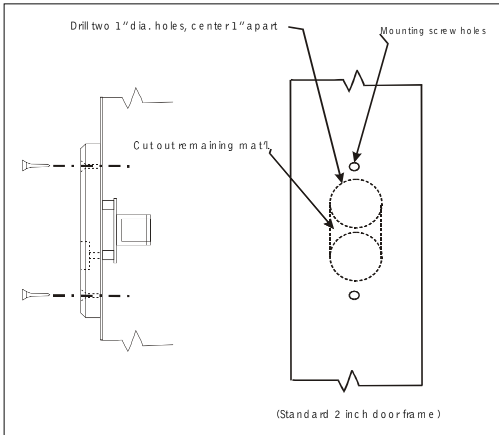
Figure 12 - ComKey Reader Installation
