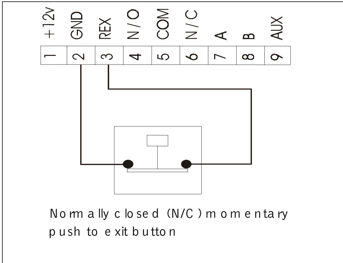
Figure 18 - Request To Exit connection
